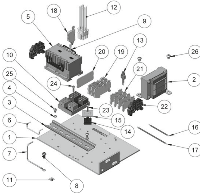
FIGURE 45. CONTACTOR PLATE ASSEMBLY FOR USE WITH DC BRAKE BHSE 3 PHASE 220/230-380/415/460-3-50/60 MODELS J, JJ, L, LL, R, & RR
