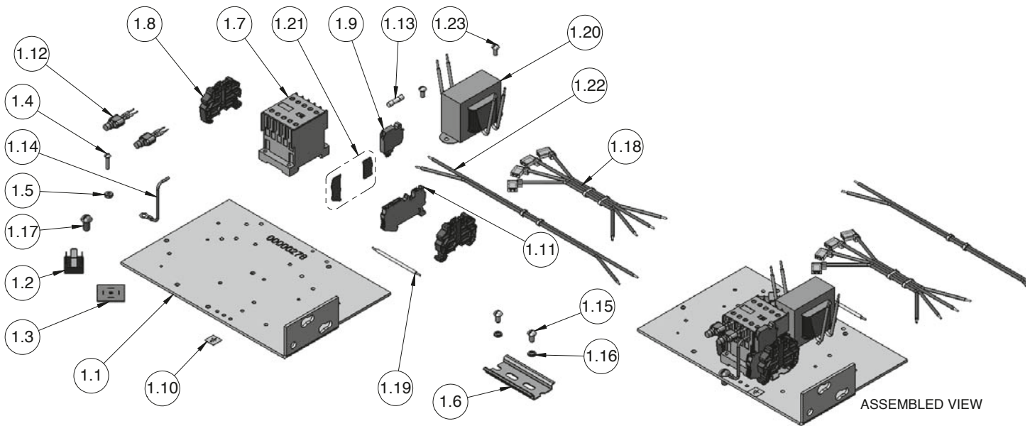
FIGURE 46. CONTACTOR PLATE ASSEMBLY FOR USE WITH DC BRAKE DIRECT CONTROL 380/415/460-3-50/60 MODELS J, L, LL, R, & RR
